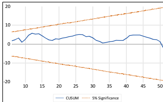
Figure 2: CUSUM Test
