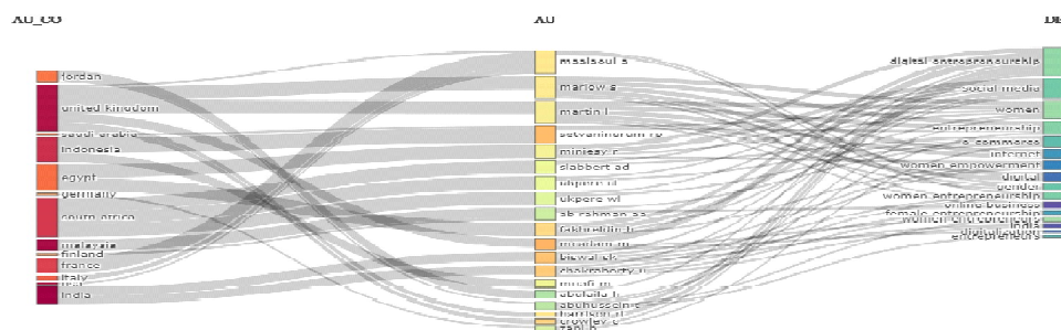
Figure 3: Three-Field Plot
