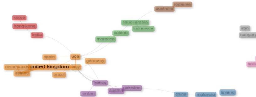
Figure 8: Collaboration Network
